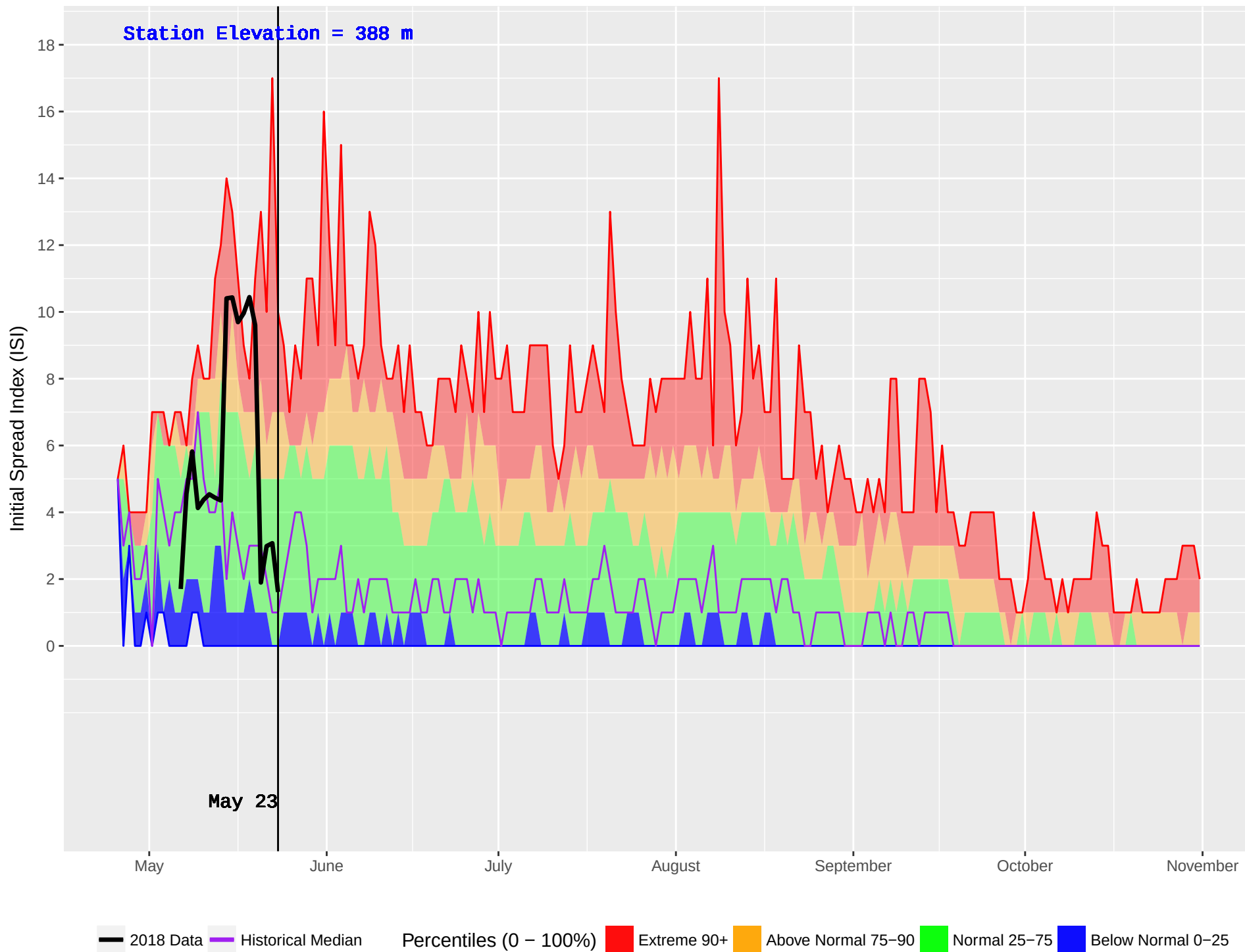
BELL-IRVING (432) : Historical (1986–2016) and Current (2018) Noon Initial Spread Index (ISI)
